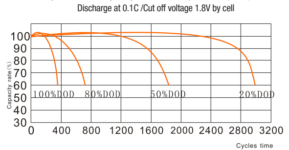
Cycle life curves (25°C) / Courbes de cycle de vie (25°C)
